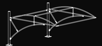
PERSPECTIVE VIEW
